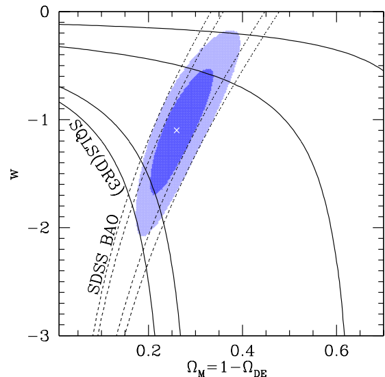
FIG. 3.— Contours at 1\sigma and 2\sigma confidence levels (estimated from \Delta\chi^2 = 2.3 and 6.17 ) are plotted in the \Omega_{\text{M}}-w plane. Solid lines indicate the constraint from the SQLS DR3, whereas dotted lines are from the baryonic acoustic oscillations (BAO) detected in the SDSS luminous red galaxy power spectrum (Eisenstein et al. 2005). The joint constraint from SQLS and BAO are shown by shaded regions: The best-fit model (\Omega_{\text{M}}, w) = (0.26, -1.1) is indicated with a cross.
