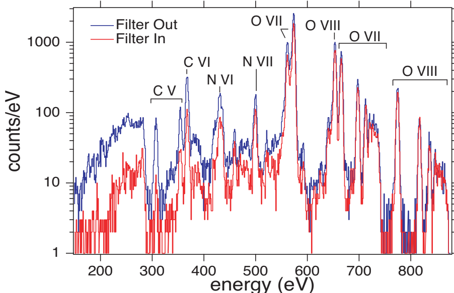
FIG. 1: Comparison of spectra measured with the VSG filter in and filter out in the 150 to 900 eV energy band measured with the ECS.
