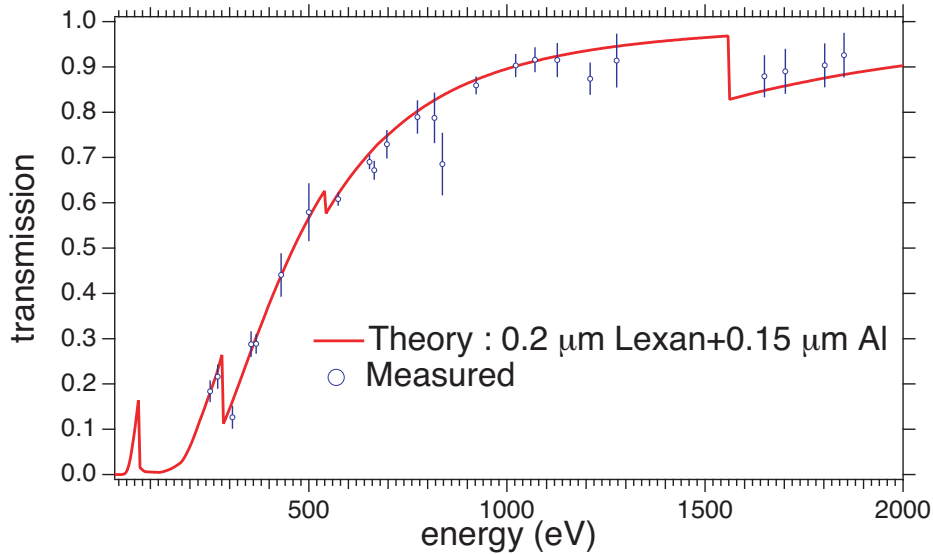
FIG. 2: Transmission of a blocking filter manufactured by the Luxel corporation. All the data points on were acquired in a total of six hours.
