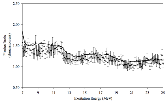
FIGURE 2. The surrogate ratio \left(\frac{^{234}\text{U}(\alpha, \alpha'f)}{^{236}\text{U}(\alpha, \alpha'f)}\right) is shown in the solid black points as obtained from this experiment. The solid line is the ENDF-B7 data for the \frac{^{233}\text{U}(n, f)}{^{235}\text{U}(n, f)} ratio. The error bars represent statistical error only. Please note the suppressed ordinate axis.
