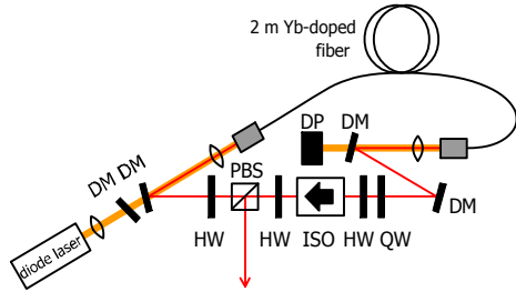
Figure 1. Schematic diagram of a grating-less fiber oscillator: HW, half-wave plate; QW, quarter-wave plate; ISO, isolator; PBS, polarizing beam splitter; DP, beam dumper; DM, dichroic mirror.
