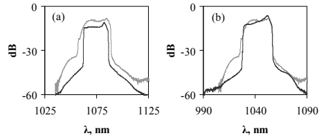
Figure 2. (a) Spectrum of 9 nJ (black) and 25 nJ pulses (gray) from grating-compensated oscillator. (b) Spectrum of 25 nJ pulses from grating-less compensator (black) and grating-compensated oscillator. The latter is the same data as in (a), scaled to the center wavelength of the grating-less oscillator.
