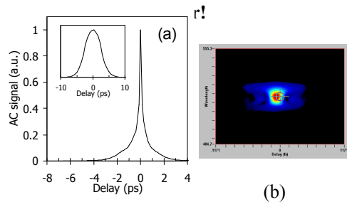
Fig. 3. (a) Intensity autocorrelation trace after the compression. Inset, autocorrelation trace of chirped output pulses (b) FROG trace after the compression
