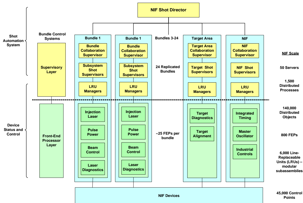
Figure 1 Bundle-based partitioning
