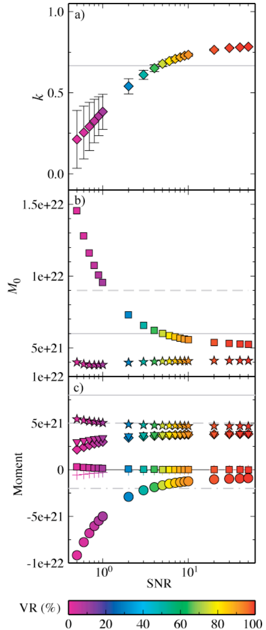
Figure 6. A noisy synthetic composite event at a depth of 400 m is inverted using Green's functions for an event at 1 km. a) Source-type parameter k , where the theoretical value is given by the grey line. b) M_0 (square) and M_{ISO} (star), where the theoretical values are given by the dashed and solid grey lines, respectively. c) M_{33} (star), M_{13} (cross), M_{23} (circle), M_{11} (diamond), M_{22} (triangle) and M_{12} (square) where theoretical values are given by the grey lines. Symbol color is the variance reduction (VR) of the solution.
