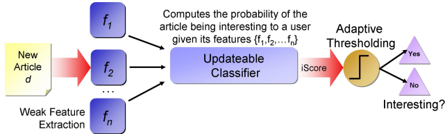
Figure 1: iScore architecture.
