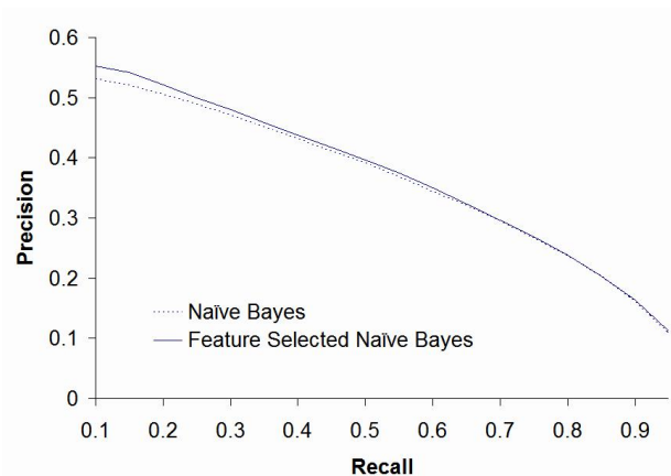
Figure 5: Precision recall curve of the classifiers.
