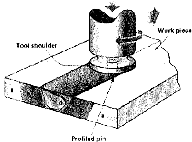
Figure 1. Schematic of the Friction Stir Joining Process. The pin tool is rotated and translated along the joint resulting in the plasticizing of the base metals and their subsequent mechanical intermixing.
