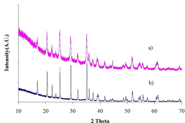
Figure 2. X-ray diffraction patterns of a) nanometric \text{LiMnPO}_4 made by combustion synthesis and b) hydrothermally prepared sub-micron \text{LiMnPO}_4 .
