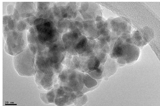
Figure 1. TEM image of nanosized \text{LiMnPO}_4 by combustion synthesis
