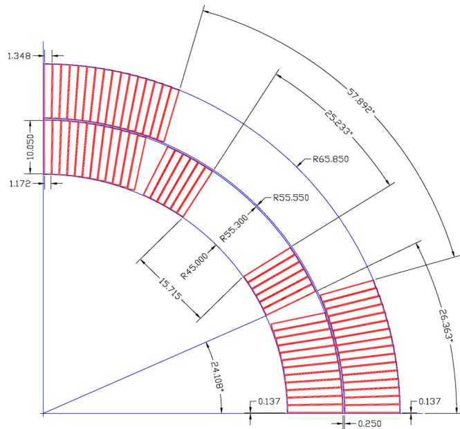
Fig. 2. TQ and LQ coil cross section.
