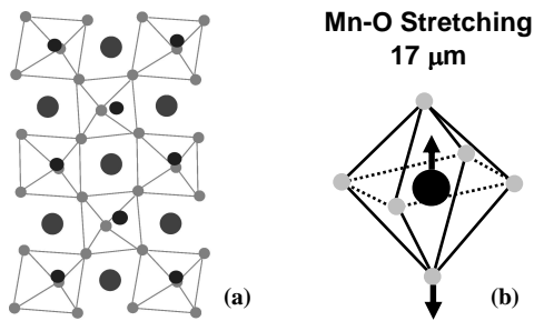
Fig 1. (a) Distorted orthorhombic structure of \text{Pr}_{0.7}\text{Ca}_{0.3}\text{MnO}_3 . (b) Atomic displacements within the \text{MnO}_6 octahedra associated with the 17\ \mu\text{m} ( 580\ \text{cm}^{-1} ) phonon mode which modulates the Mn-O distance and hence the tolerance factor.
