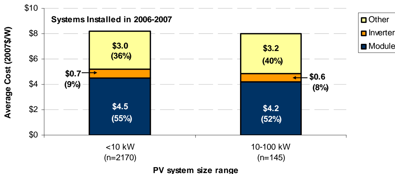
Figure 15. Module, Inverter, and Other Costs
