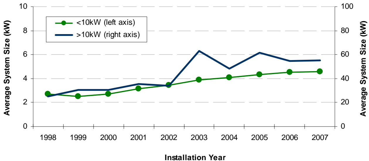
Figure 10. PV System Size Trends over Time
