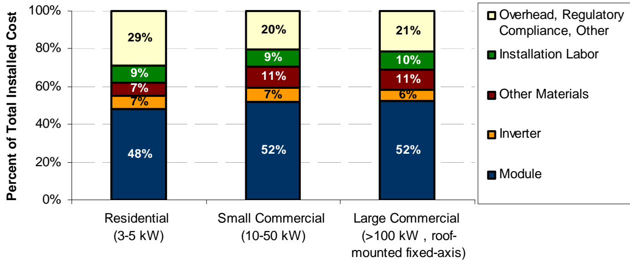
Figure 16. Results from Survey of PV Installers on Component Costs
