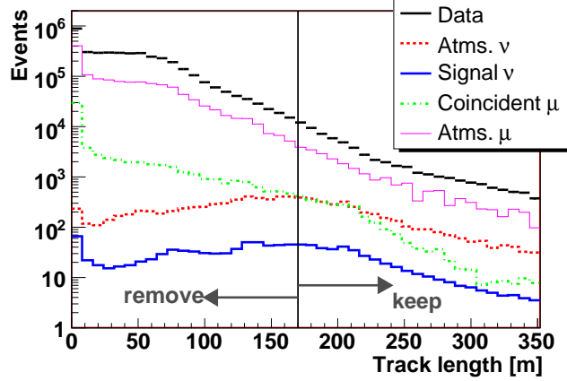
FIG. 11: The reconstructed track length within the detector is shown. In order to identify muon neutrino tracks, events were required to have long tracks of at least 170 meters. This removed a large fraction of the atmospheric muon simulation, but had a smaller effect on the atmospheric neutrino and signal simulations.
