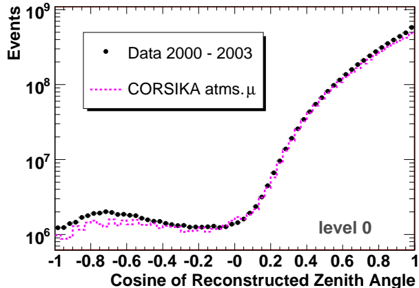
FIG. 1: The cosine of the reconstructed zenith angle is shown for every event at the beginning of the analysis (level 0). The experimental data is dominated by downgoing atmospheric muons. Events reconstructed as upgoing appear on the left side of the plot and downgoing events appear on the right.
