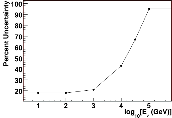
FIG. 12: The estimated uncertainty in the atmospheric neutrino flux as a function of energy. Due to the large uncertainty in the prompt neutrino flux at greater than 10^4 GeV, the total uncertainty rises sharply.
