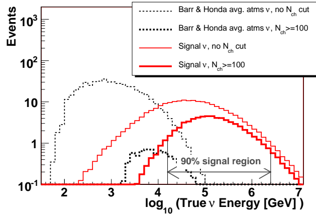
FIG. 5: The true energy of the simulation is shown for atmospheric neutrino and signal events. The thin dashed (atms. \nu ) and solid (signal \nu ) curves represent the number of events before the N_{\text{ch}} \geq 100 requirement. The thick dashed and solid lines represent only the events in the high energy sample.
