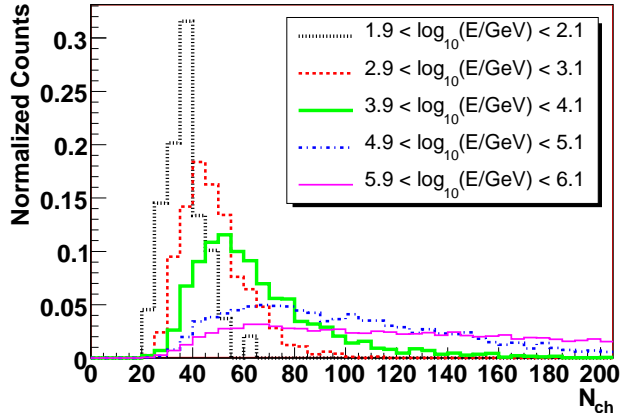
FIG. 2: The number of OMs hit during an event ( N_{\text{ch}} ) was used as an energy-correlated observable. Each line on this N_{\text{ch}} distribution represents events with approximately the same simulated energy. High energy events may not be contained within the detector and hence can trigger a wide N_{\text{ch}} span.
