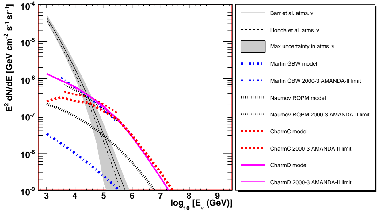
FIG. 10: Prompt neutrino models and upper limits based on this analysis. The Barr et al. and Honda et al. atmospheric neutrino predictions are shown for reference. Two charm models [34] were tested, along with the Naumov RQPM [31, 32] and Martin GBW [30] models.
