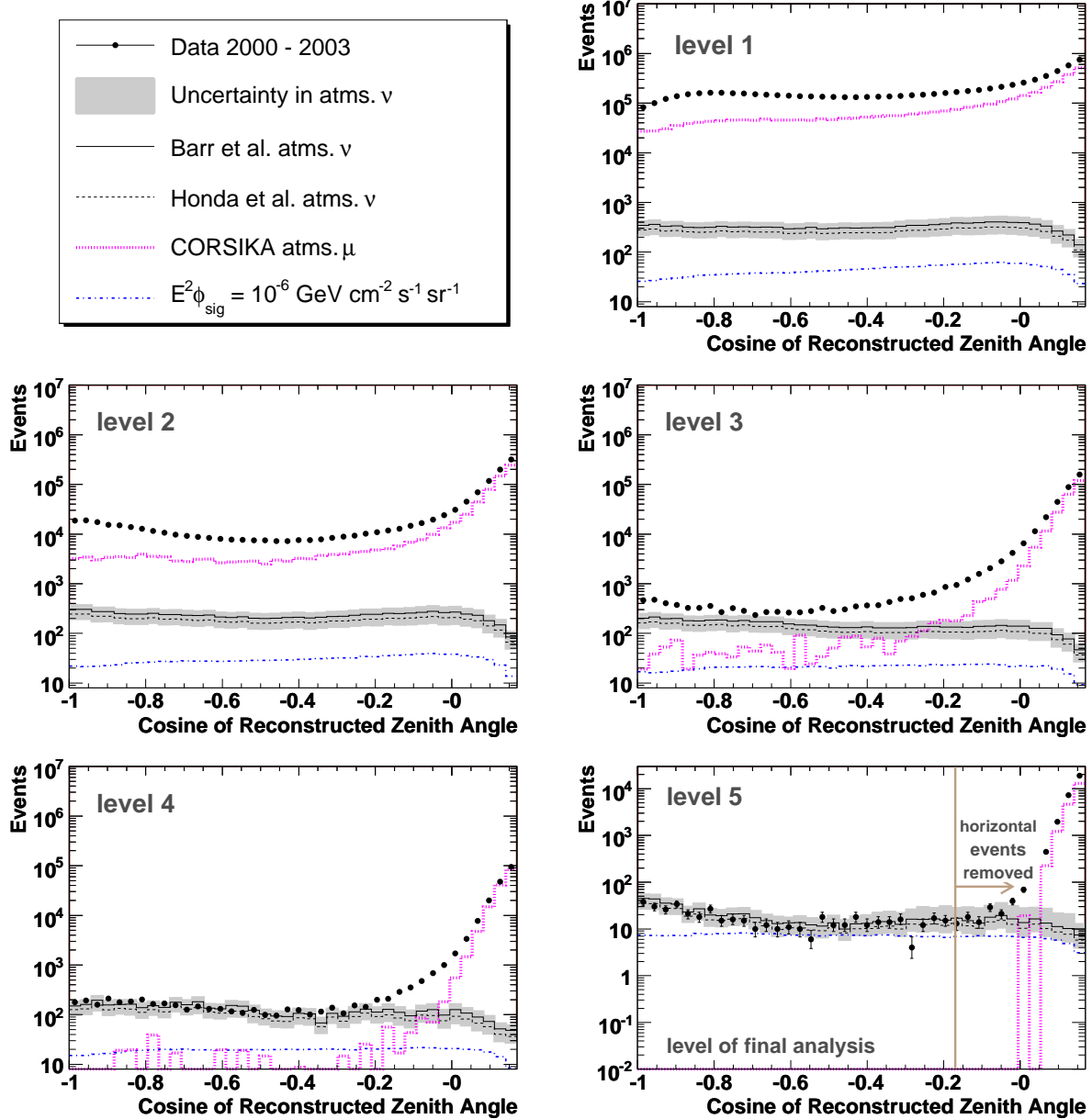
FIG. 3: The cosine of the zenith angle is plotted for all events surviving the event quality criteria at a given level. Events at \cos(\text{zenith}) = -1 are traveling straight up through the detector from the Northern Hemisphere. The initial zenith angle requirement removed events from 0^\circ to 80^\circ (level 1 - top right). Events reconstructed just above the horizon appear at the right side of each plot. Each level represents an increasingly tighter set of quality requirements. As the quality level increased, misreconstructed downgoing muons were eliminated. To ensure a clean upgoing sample, events coming from the horizon were discarded by requiring reconstruction angles greater than 100^\circ . The final analysis was performed at level 5 (bottom right) with horizontal events removed.
