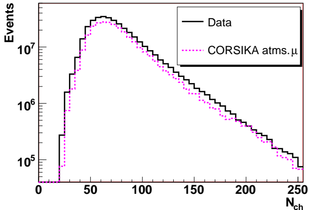
FIG. 7: In the inverted analysis, the highest quality downgoing events were studied. The N_{\text{ch}} distribution is shown for all events which survive the inverted quality requirements.
