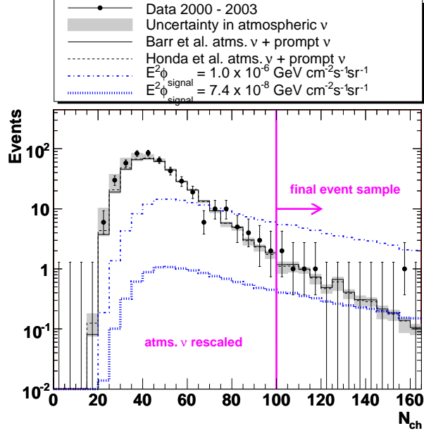
FIG. 4: N_{\text{ch}} , or number of OMs hit. Prediction for both conventional and prompt atmospheric neutrinos are shown and their uncertainties are represented by the gray band. The central prompt neutrino flux used here is the average of the Martin GBW [30] and Naumov RQPM [31, 32] models. All atmospheric neutrinos are normalized to the number of data events in the range 50 < N_{\text{ch}} < 100 . The lower signal flux curve corresponds to the limit obtained in this paper.
