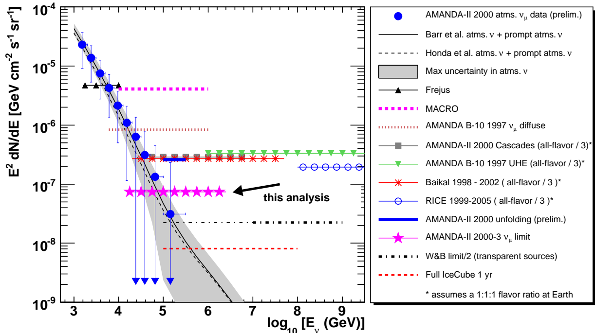
FIG. 8: The upper limits on the \nu_\mu flux from sources with an E^{-2} energy spectrum are shown for single and all-flavor analyses. All-flavor upper limits have been divided by three, assuming that the neutrino flavor ratio is 1:1:1 at Earth. The Fréjus [12], MACRO [13], and AMANDA-B10 [10] upper limits on the \nu_\mu flux are shown, as well as the unfolded atmospheric spectrum from 2000 AMANDA-II data [42]. The AMANDA-II all-flavor limit from 2000 [11], the AMANDA-B10 UHE limit [43], the Baikal five year limit [14] and the RICE six year limit [44] have all been adjusted for the single flavor plot. The \Phi \propto E^{-2} limit from this analysis is a factor of four above the Waxman-Bahcall upper bound. Although not shown, this analysis excludes the \Phi \propto E^{-2} predictions made by Nellen, Mannheim and Biermann [4] and Becker, Biermann and Rhode [5] and constrains the MPR upper bound for optically thick pion photoproduction sources [6]. The IceCube sensitivity for a full detector was estimated with AMANDA software [45].
