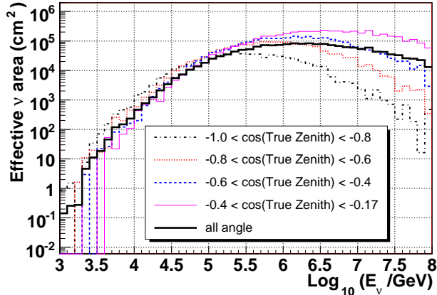
FIG. 6: Effective area for \nu_\mu as a function of the true simulated energy at the Earth’s surface in intervals of cosine of the true zenith angle. The effective area is the equivalent area over which the detector would be 100% efficient for detecting neutrinos. The absorption of neutrinos and reduction of their energy via neutral current interactions in the Earth are taken into account. The angle-averaged effective area is represented by the solid black line.
