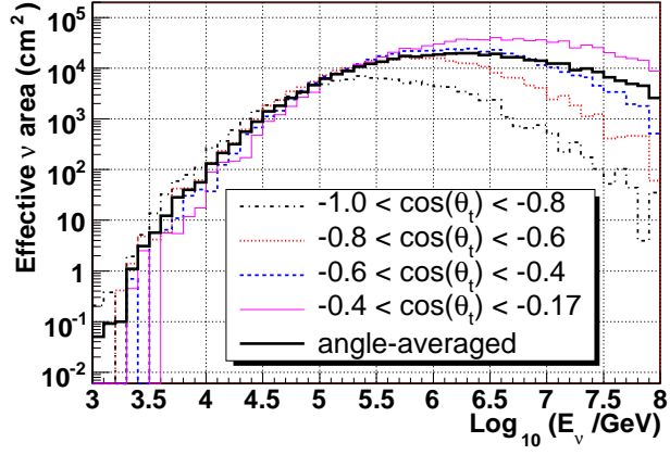
FIG. 13: Effective area for \nu_\mu as a function of the true simulated energy at the Earth's surface in intervals of cosine of the true zenith angle, \theta_t . The angle-averaged effective area is represented by the solid black line. This calculation was based on the final event sample for events satisfying N_{\text{ch}} \geq 100 .
