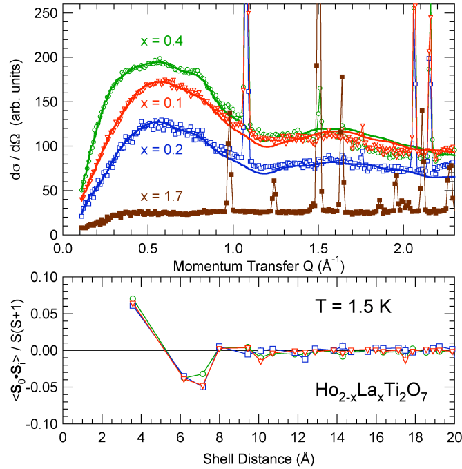
Figure 6. Diffuse magnetic scattering studied at DCS, corrected for Vanadium and monitor intensities. The energy window was set to \pm 0.1 meV. Intensity is highest at x=0.4 because of the higher sample transmission. The diffuse S(Q) has two maxima at 0.6 \text{ \AA}^{-1} and 1.6 \text{ \AA}^{-1} , respectively. The upper panel also shows the fits, and the lower panel shows the resulting time averaged spin correlations in the near neighbour shells, from a reverse Monte Carlo simulation.
