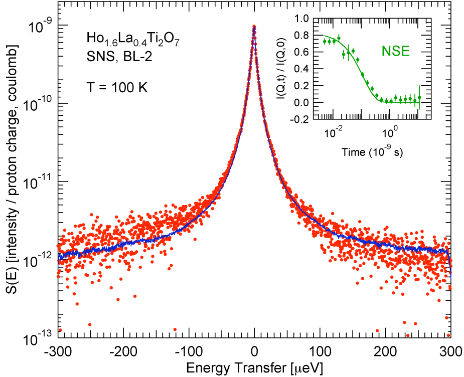
Figure 7. BS and NSE data and fits combined at T = 100 K for the x = 0.4 sample. For details, see text.
