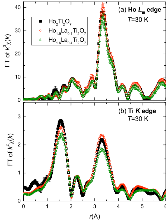
Figure 5. (Color online) (a) FT amplitudes of the k^3\chi(k) EXAFS data from the Ho L_{\text{III}} edge and (b) the FT of the k^2\chi(k) of data from the Ti K edge for the x=0, 0.1 and 0.4 samples, all at T=30 K. Transform ranges are as in figure 4.
