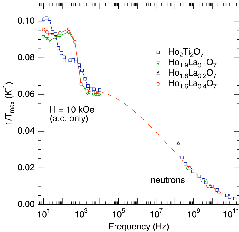
Figure 9. Combination of results from AC susceptibility (top left) and quasielastic neutron scattering (bottom right) measurements. For susceptibility, this graph shows the inverse of the temperatures at which the main maximum in the imaginary part occurs, as a function of the probing frequency, for the x = 0 , x = 0.1 and x = 0.4 samples. For the neutron data, the inverse measurement temperature is plotted against the inverse of the main spin relaxation time as fitted from either NSE or NSE and backscattering combined. Symbols used: x = 0 ( \square ), x = 0.1 ( \nabla ), x = 0.2 ( \triangle ), x = 0.4 ( \circ ). The slope of the curve of the neutron data corresponds to an activation energy in the Arrhenius law of \Delta \sim 290 K.
