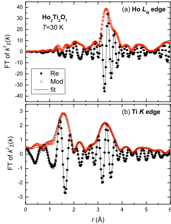
Figure 4. (a) FT of the k^3\chi(k) EXAFS data from the Ho L_{\text{III}} edge and (b) the FT of the k^2\chi(k) of T=30 K data from the Ti K edge of pure \text{Ho}_2\text{Ti}_2\text{O}_7 are shown together with fits. Transform ranges are between 2.5-14.4 Å -1 and 3.5-11.4 Å -1 respectively, all Gaussian broadened by 0.3 Å -1 . Error bars are based on the reproducibility over multiple scans.
