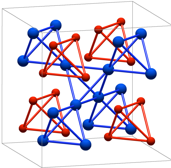
Figure 1. A unit cell of the cubic pyrochlore structure showing the rare earth (large blue spheres) and titanium (small red spheres) sublattices.
