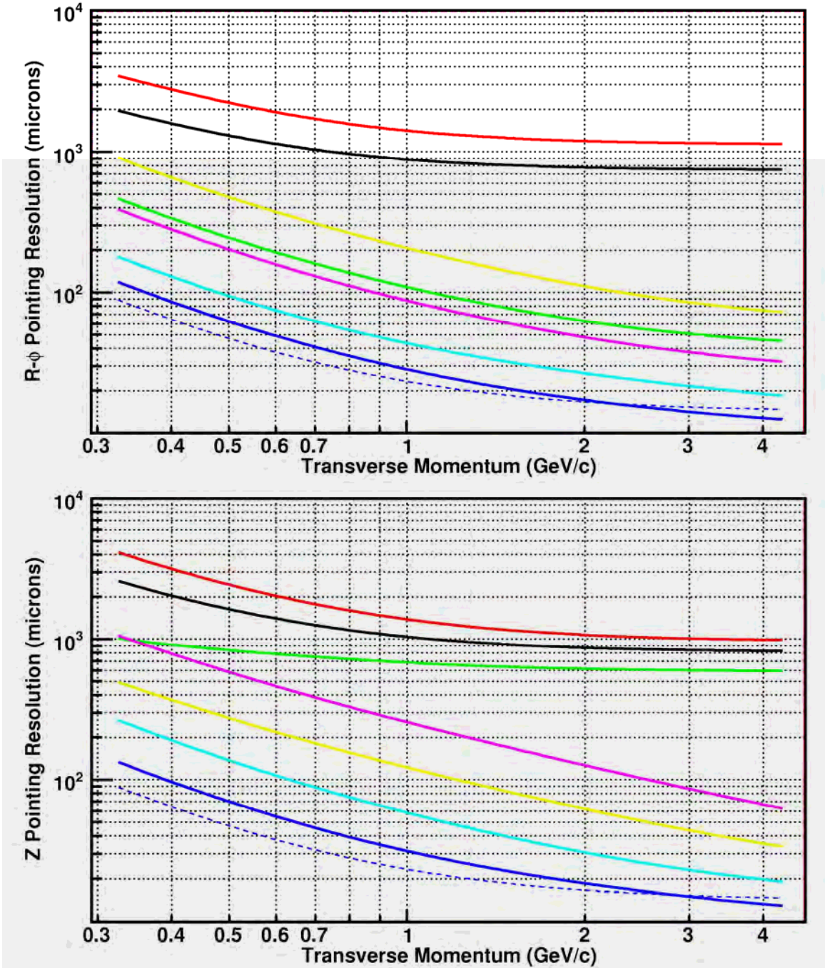
Figure 23: The pointing resolution of each element of the HFT detector system ( \sigma ); where the r - \phi and z pointing resolutions are plotted separately (top and bottom, respectively). The calculations assume a kaon passing through the system. Data at 750 MeV/c is a useful line of reference to guide the eye. The pointing resolution of the TPC onto the vertex is shown by the red line. The pointing resolution of the TPC onto the SSD is shown by the black line. The TPC+SSD pointing at IST2 is shown in green. The TPC+SSD+IST2 pointing at IST1 is yellow, TPC+SSD+IST2+IST1 pointing at PIXEL2 is magenta, TPC+SSD+IST2+IST1+PIXEL2 pointing at PIXEL1 is cyan, and the full system TPC+SSD+IST2+IST1+PIXEL2+PIXEL1 pointing at the vertex is blue. The blue dashed line is the idealized HFT performance from Equation 1; without beam pipe or other sources of MCS.
