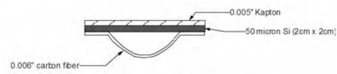
Figure 50: A cross-section of the prototype detector ladder showing its structure and materials.
