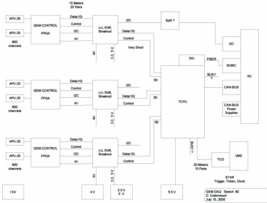
Figure 79: Schematic design of the APV25 chip readout system and STAR DAQ integration based on the FGT prototype setup.
