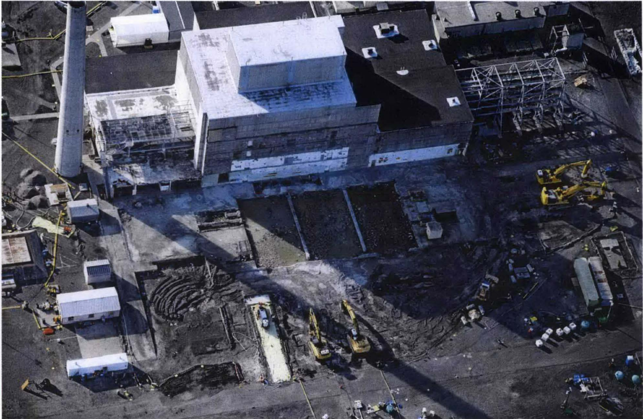
Fig. 4. The superstructure has been completely removed to slab-on-grade.
