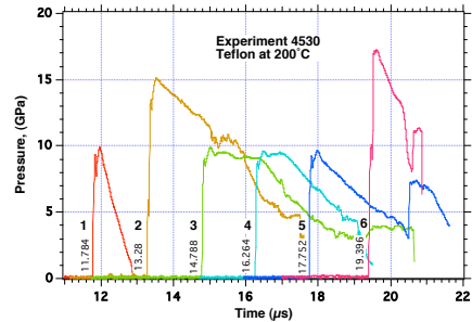
FIGURE 4. Pressure gauge traces for the heated Teflon experiment where the target was subjected to dynamic loading of 9.53 GPa by an Aluminum flyer plate impacting it with a velocity of 1.82 mm/μs.
