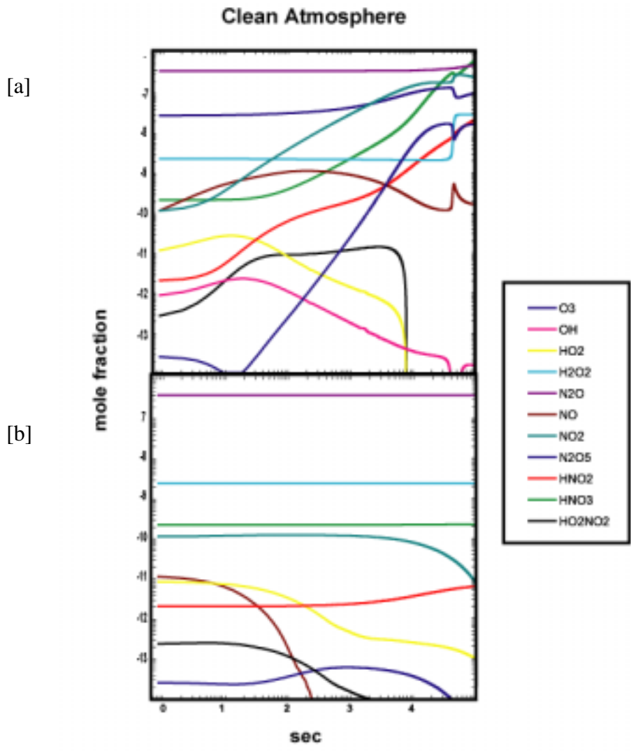
Figure 3. Molecular species concentrations (mole fraction vs. seconds) in a clean background regime, full solar cycle. [a] with ionizing radiation [b] without ionization
