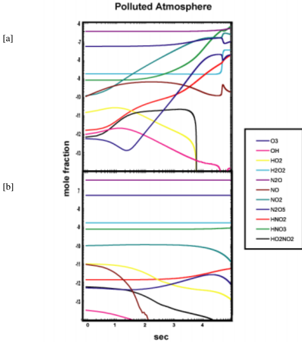
Figure 4. Molecular species concentrations (mole fraction vs. seconds) in a polluted background regime, full solar cycle. [a] with ionizing radiation [b] without ionization
