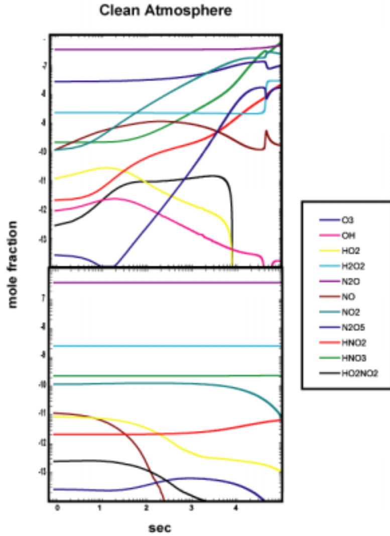
Figure 2. Molecular species concentrations (mole fraction vs. seconds). [a] with 1.05 \times 10^9 ion pairs / \text{cm}^3 flux. [b] without ionization.
