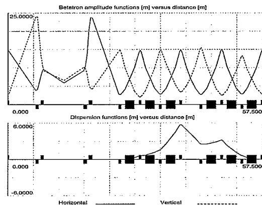
Figure 2: The lattice functions for one RCS super-period
