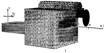
Figure 5: 3D OPERA model for the entrance end of the Lambertson magnet
