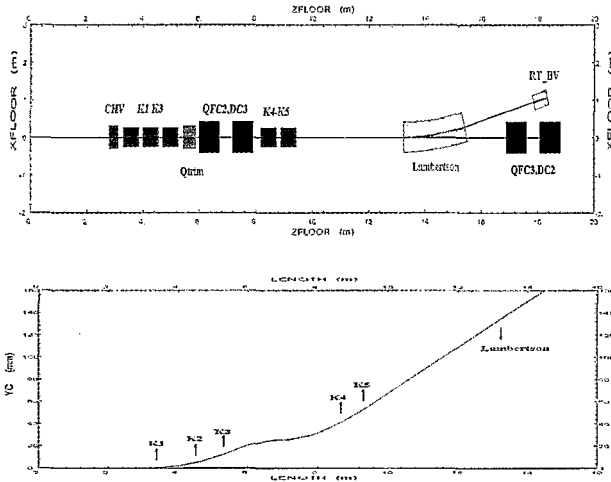
Figure 3: Layout of the extraction system and orbit displacement
