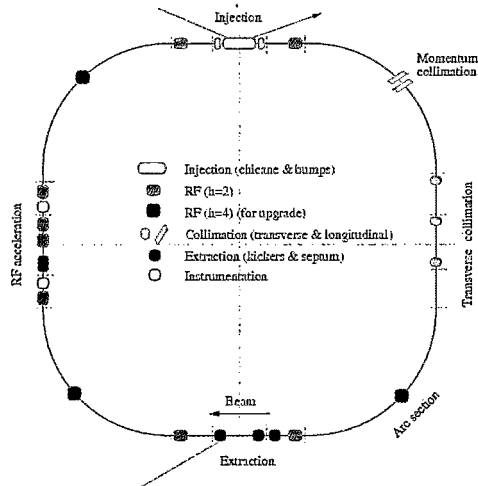
Figure 1: RCS layout and functions
