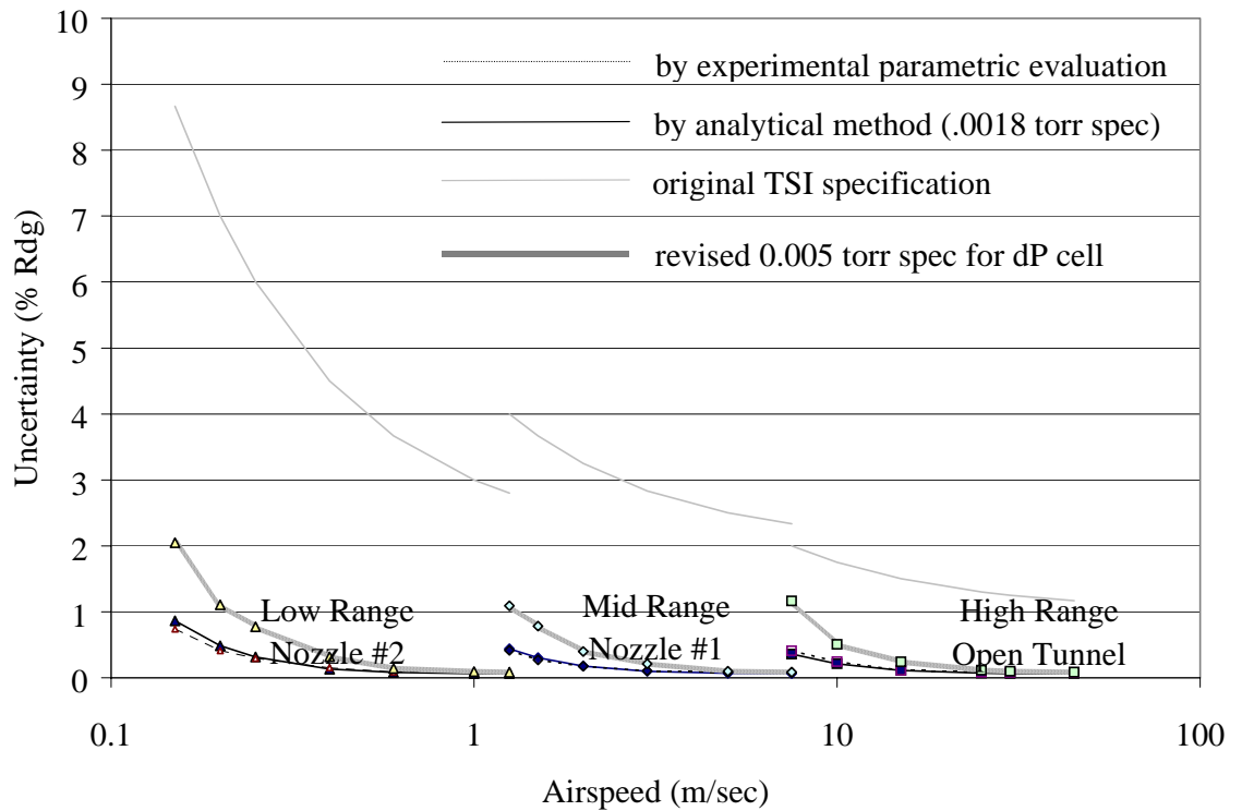
Figure 7. Static uncertainty of wind tunnel package based on manufacturer specification of instruments (experimental and analytical curves) and based on calibration of the differential pressure unit using field standard Hooke Gages (revised 0.005 torr curve). Note, overall manufacturer’s uncertainty for the wind tunnel (original TSI specification).
