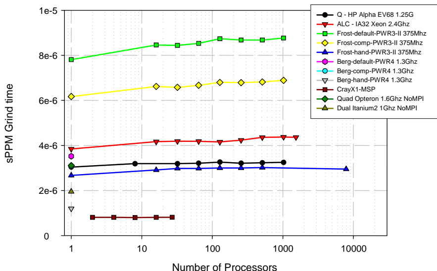
Figure 15: sPPM performance results on a scaled problem where the vertical axis represents the time to solution for one timestep of sPPM.
