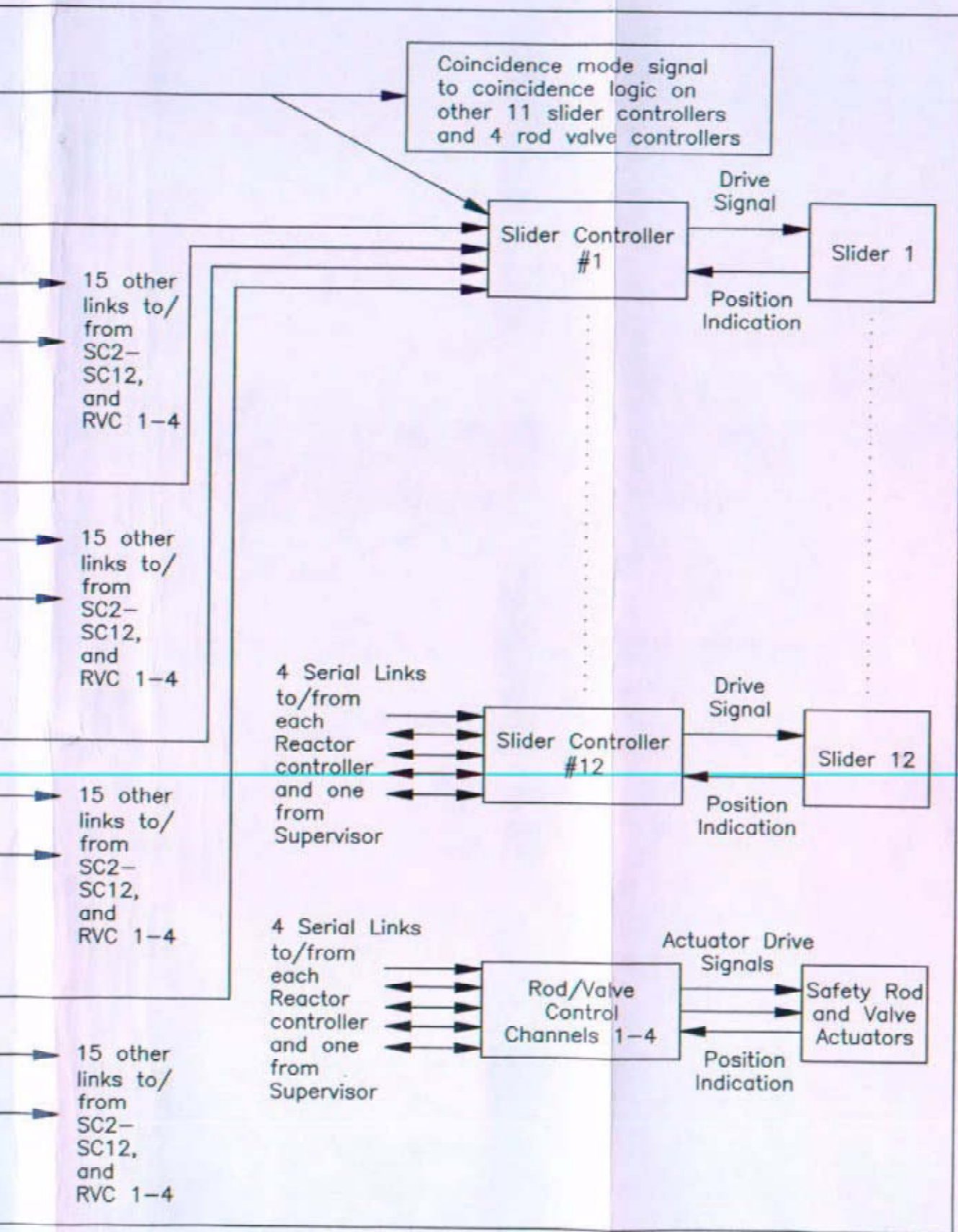
Conceptual I&C System Architecture
