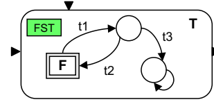
c). Transducer Template T(F)
