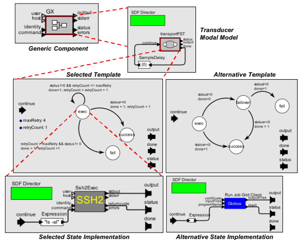
Figure 5: The Generic eXecution component
