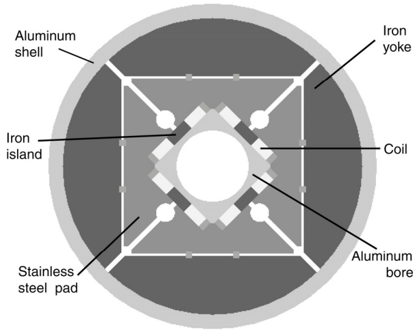
Fig. 1. SQ01 magnet cross-section
