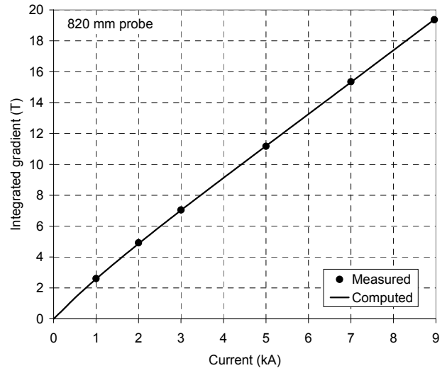
Fig. 7. Integrated gradient (T) at 22 mm radius along a 820 mm probe as a function of the current (kA): field measurements (markers) and computations (solid line).
