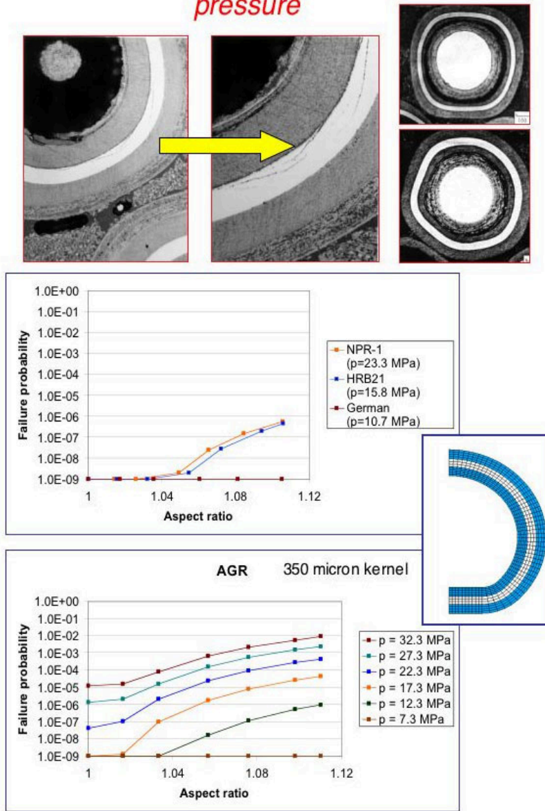
Figure 15. Effect of particle asphericity on failure probability.
