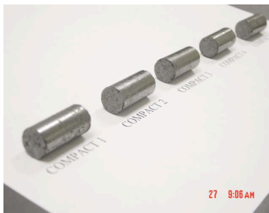
Figure 8. Compacts produced using ORNL thermosetting resin process.
