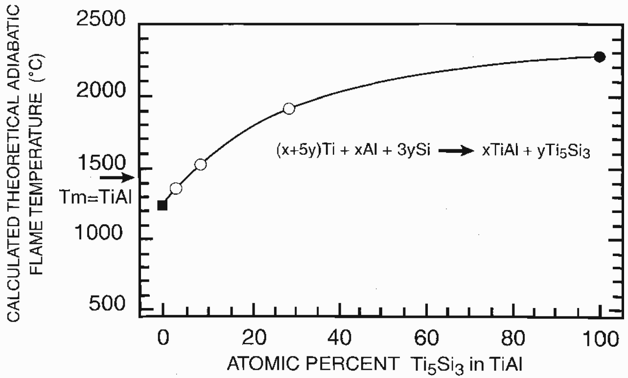
Figure 9. Calculated adiabatic flame temperatures for the reaction to form TiAl+Ti_5Si_3 insitu composites from elemental constituents, as a function of Ti_5Si_3 content.
