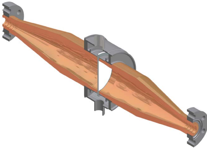
Figure 3. Configuration of proposed barrier window. Shown are mode-mixing up- and down-tapers to the \sim 63 -mm diameter alumina window from 15-mm diameter TE_{01} mode circular waveguide, grooved matching elements at entry and exit to the tapers, and a rigid supporting plenum that provides pump-out access to both sides of the window through holes not shown in the drawing.
