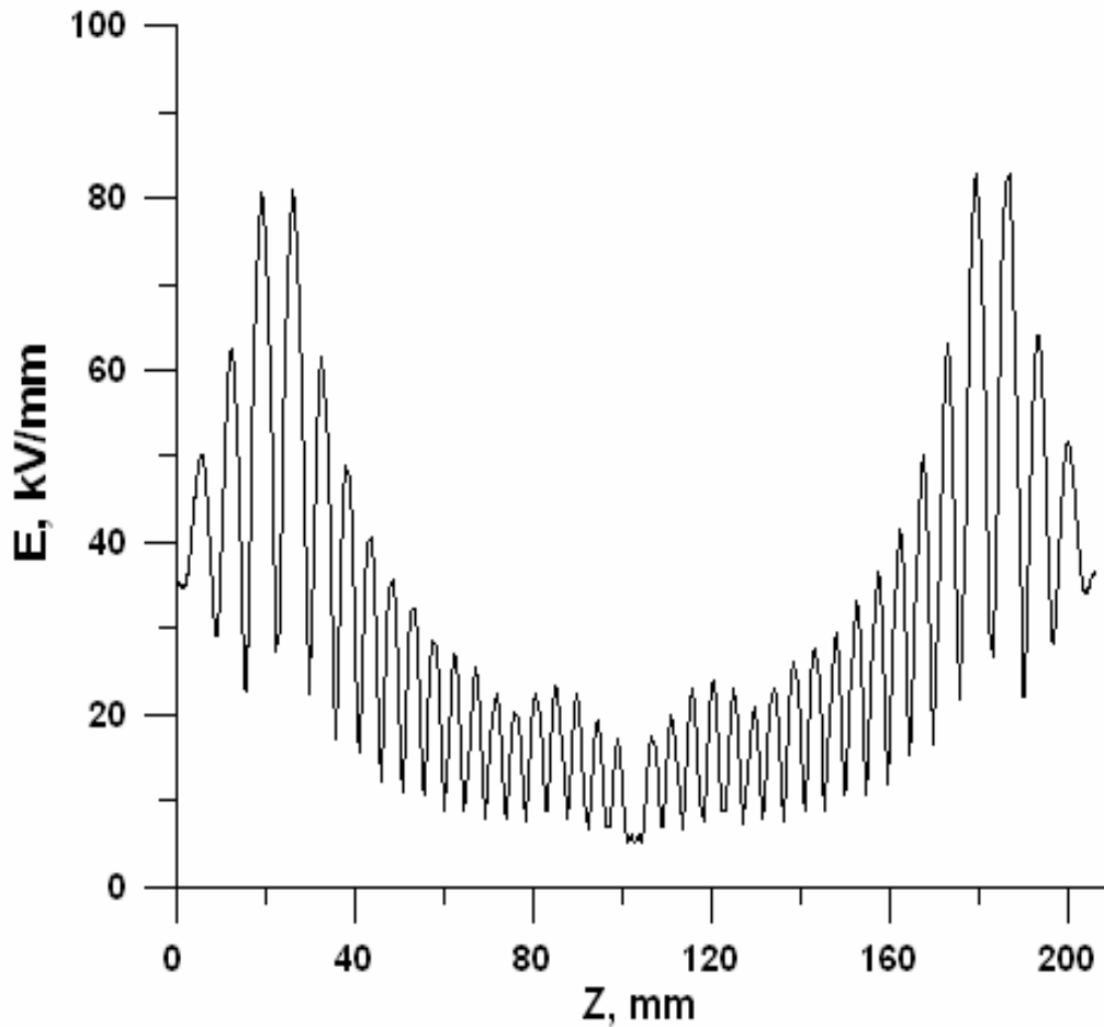
Figure 17. Calculated electric field amplitude distribution in the window-mock-up at 34.272 GHz
