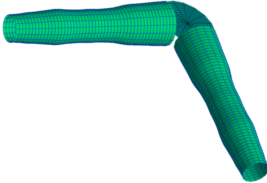
Figure 25. 3D-view of the miter bend internal surfaces – two tapers and flat mirror.
