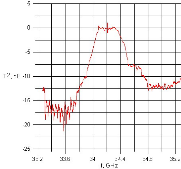
Figure 21. Measured transmission coefficient characteristics.
