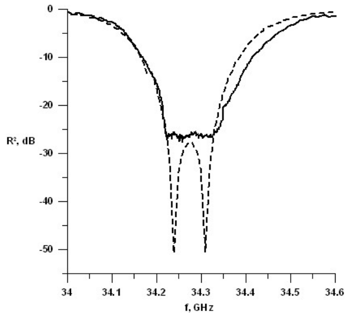
Figure 20. Calculated and measured reflection coefficient characteristics. Ceramics is BK 100-1. Disk thickness 3.6 \pm 0.01 mm, \varepsilon = 9.5 , loss tangent 2 \cdot 10^{-4} . Solid line – measured, dashed line – calculated.
