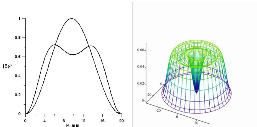
Figure 15. Intensity of electric field on the window surface for the optimized TE_{01}-TE_{02}-TE_{03} mode mixture and pure TE_{01} mode. The ratio of the maximum intensities is 1.4:1. 3-D view of the field intensity on the surface is shown on the right picture.
