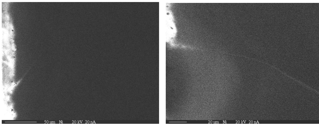
Figure 1. Nickel penetration into a copper tricrystal specimen after 48 hours at 700^\circ\text{C} ( 0.72T_m ). The nickel source is at the left in both images, and nickel has bright contrast in these electron microprobe elemental maps. (a) Penetration of about 80\mu\text{m} , along a grain boundary. (b) Penetration exceeding 300\mu\text{m} , at a sectioning plane within 80\mu\text{m} of the GBTJ. (Micrographs by R. Narayanan.)
