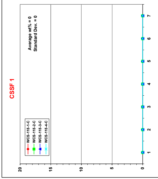
Figure A-24: Weight Percent Zirconium (Tc Segments listed bottom to top)
