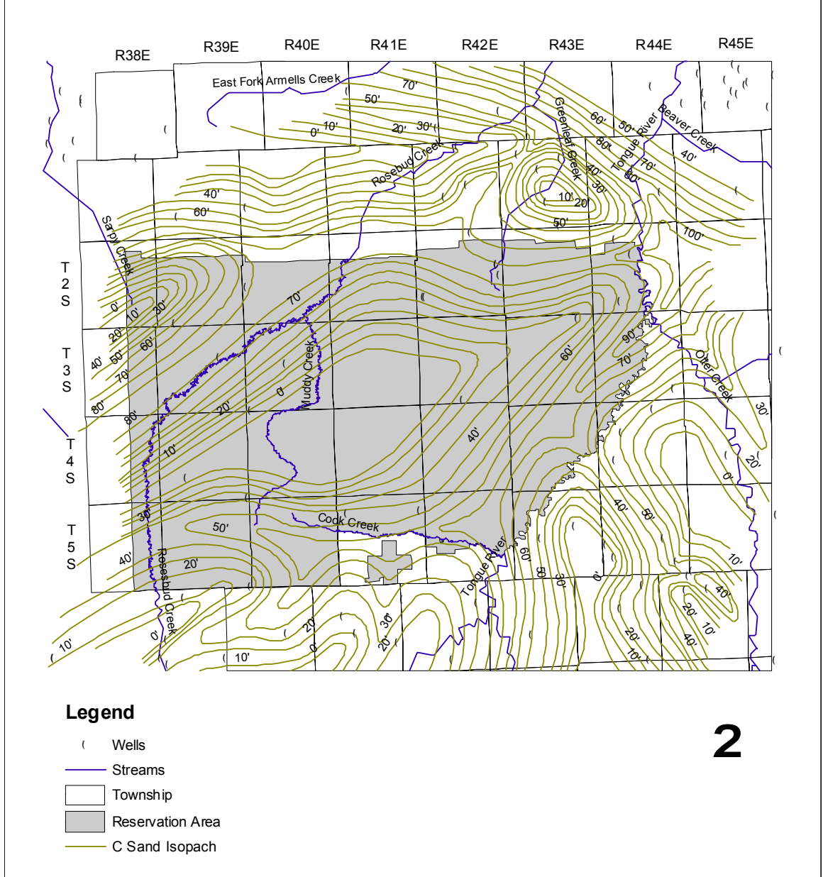
Figure 21. Isopach map of the C sandstone unit.
