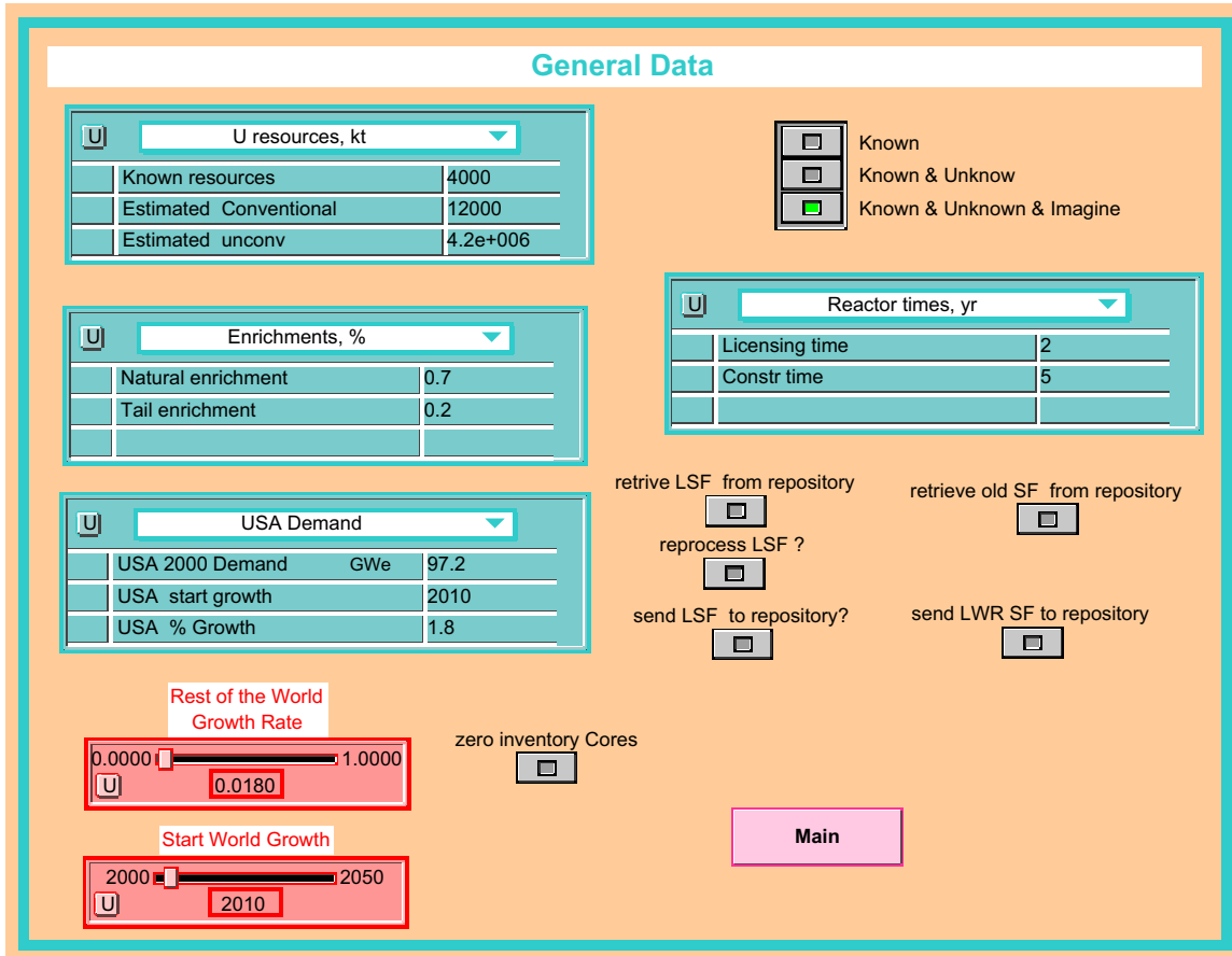
Figure 6: Interface for Changing General Model Parameters.
