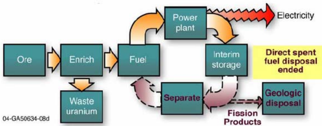
Figure 9: Continuous Recycle Strategy
