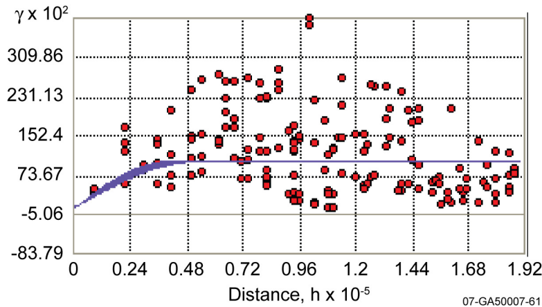
Figure 6. Variogram and best estimated function for CS-137 data. The distance is in meters.
