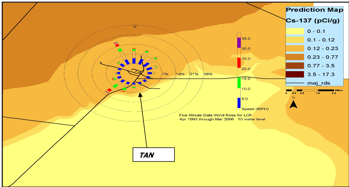
Figure 12. Disjunctive kriging prediction surface using anisotropic adjustment with georeferenced windrose over TAN facility.
