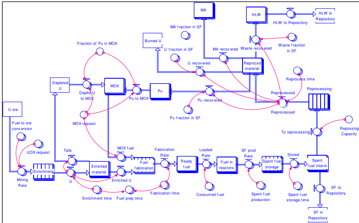
Figure 4: This Figure Shows a Simplified Version of the Complete Fuel Cycle Structure when Including Recycling.
