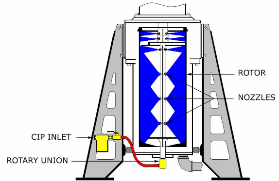
Fig. 1. Commercial contactor Clean-In-Place (CIP) design.
