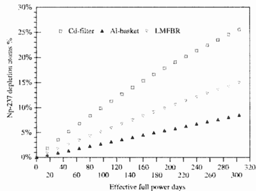
Figure 2. Comparison of the 237 Np fraction depletion (atom%) vs. EFPDs.
