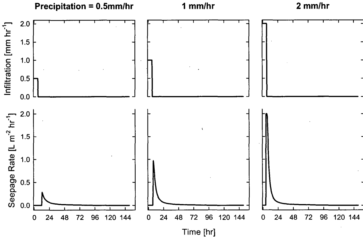
Figure 3. Infiltration rate and seepage rate for a 1D column of fracture continuum with mean fracture aperture of 100 \mu\text{m} and fracture density of 10 \text{ m}^{-1} . The simulated net precipitation (supply of water) values are 0.5, 1, and 2 mm/hr for duration of 6 hrs.
