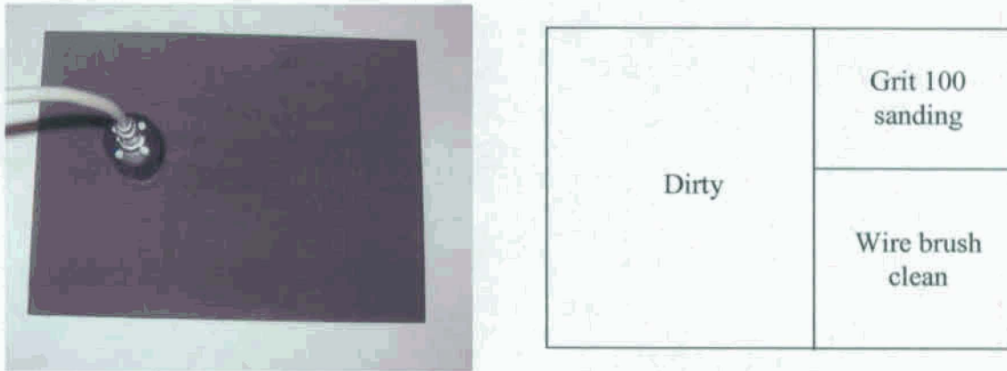
FIGURE 3. Thermally spray coated steel sample with three sections of surface preparation.
