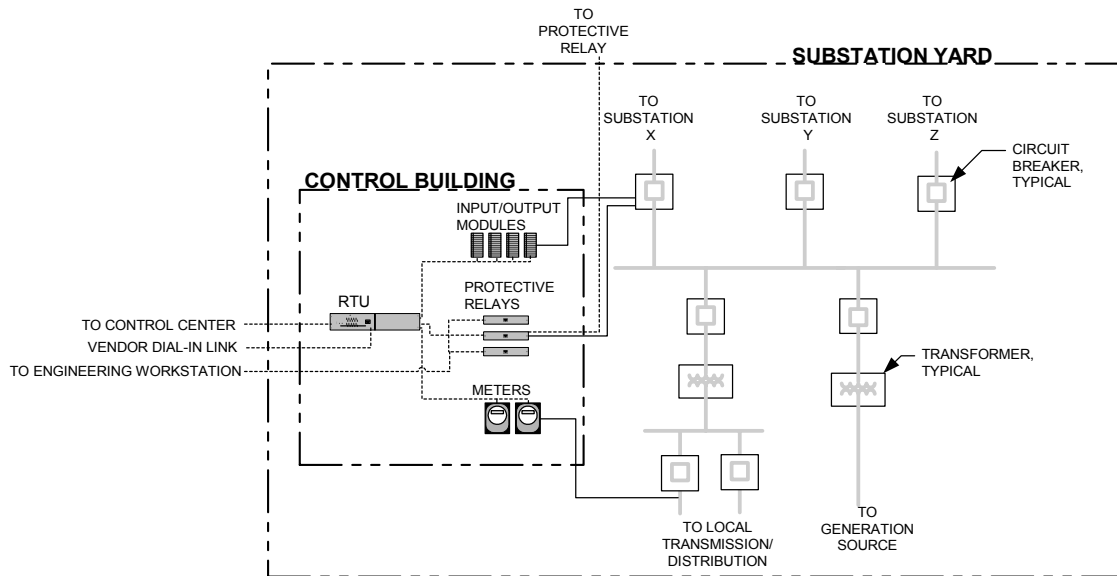
Figure 2-8. Typical transmission substation.
