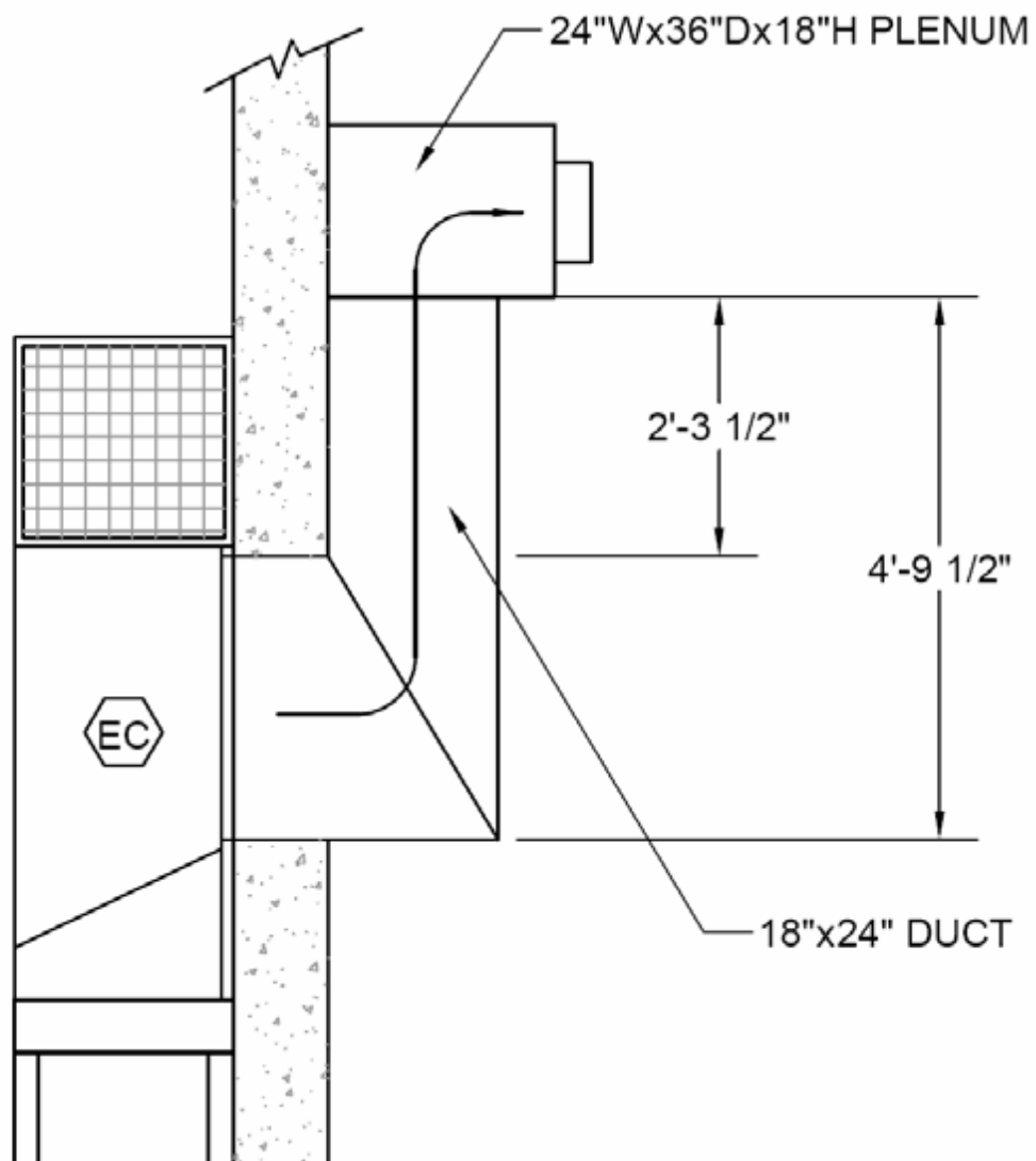
Figure 13. Supply plenum layout for Wagon OASys indirect/direct evaporative cooler
