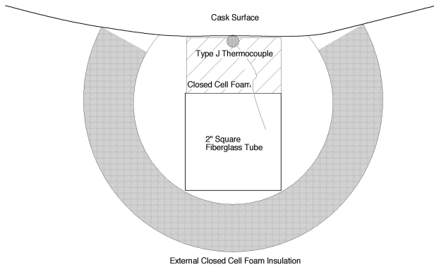
Fig. 2. Cross section of thermocouple rake.
