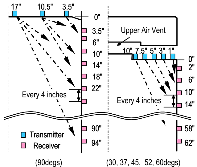
Fig. 12. Ultrasonic sensor disposition.
