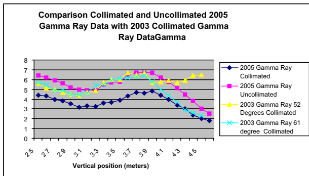
Fig. 10. Comparison of 2003 and 2005 collimated measurements.
