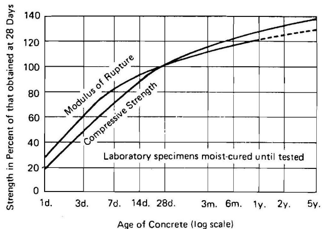
Fig. 9. Age-strength relationships for moist-cured concrete. 4
