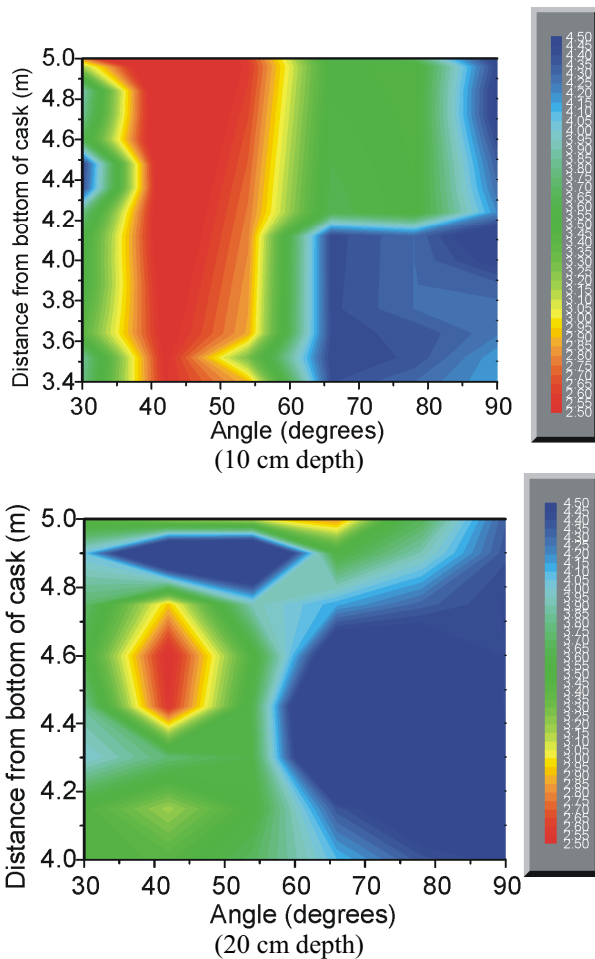
Fig. 13. Surface wave propagation distribution on upper part of VSC-17 cask (Sector 30-90 degrees).
