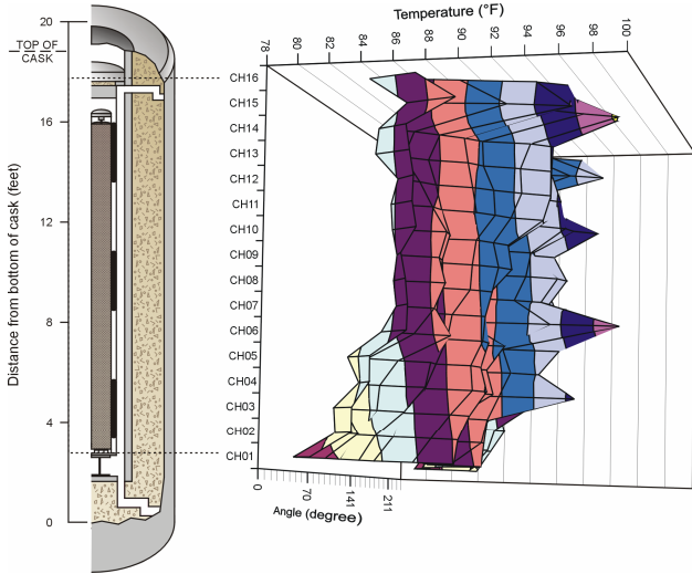
Fig. 5. Temperature readings for the 0 degree to 210 degree positions.
