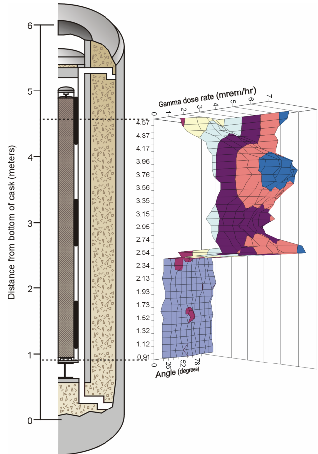
Fig. 1. Surface dose rate of the VSC-17 VCC from 0 to 90 degrees.
