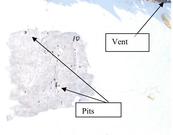
Fig. 8. Pits at position 10, below the 45-degree vent.
