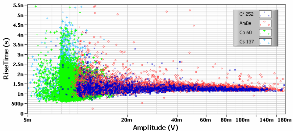
Figure 6. Combined gamma and neutron data processed with the PSD algorithm.
