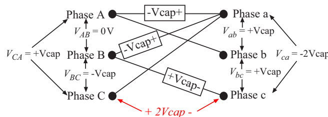
Figure 2.6: An example of invalid switching-device combination having 2V_{cap} across the non-conducting switch cells
