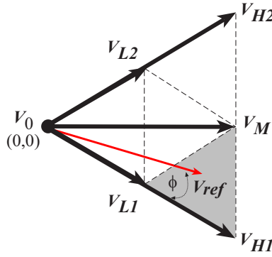
Figure 5.4: SVM for three-level switching, Case 2
