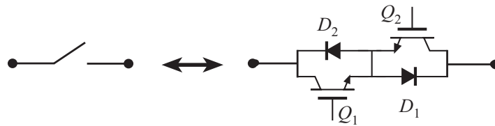
Figure 1.6: Conventional four-quadrant switch used in the matrix converter
