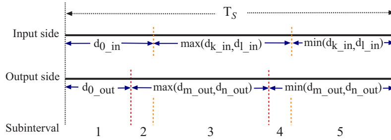
Figure 3.14: The pattern of input-side and output-side space vectors for the single-capacitor control scheme
