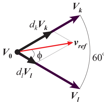
Figure 3.2: Diagram of SVM
