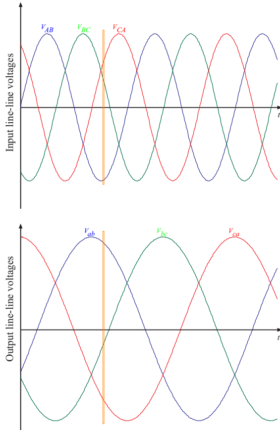
(a) Time domain
