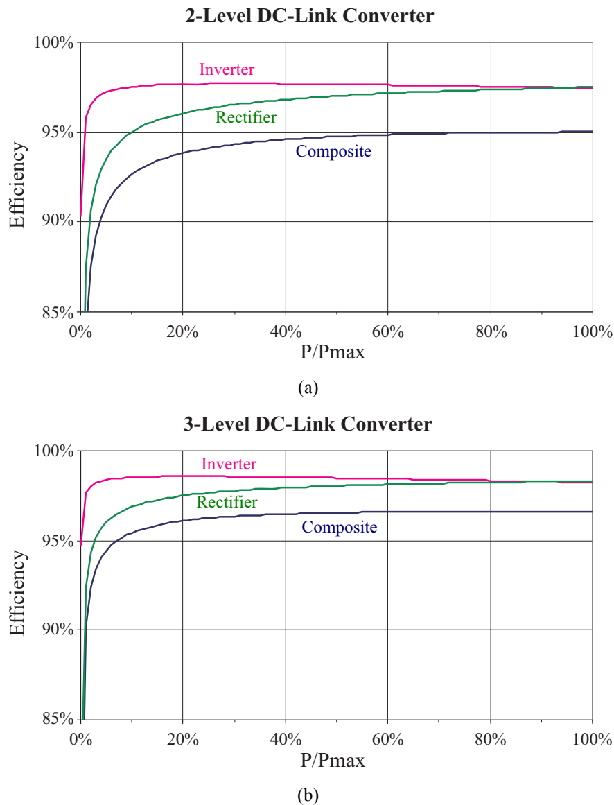
Figure 1.13: Efficiencies of three-phase DC-link converters: (a) two-level switching, (b) three-level switching
