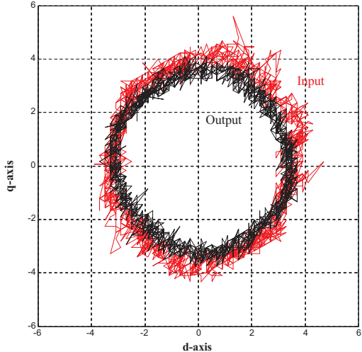
Figure 3.21: Trajectories of input- and output-currents in dq coordinate
