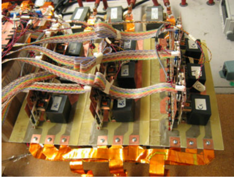
Figure 6.3: Power stage consisting of three printed circuit boards; each PCB contains three H-bridge switch cells
