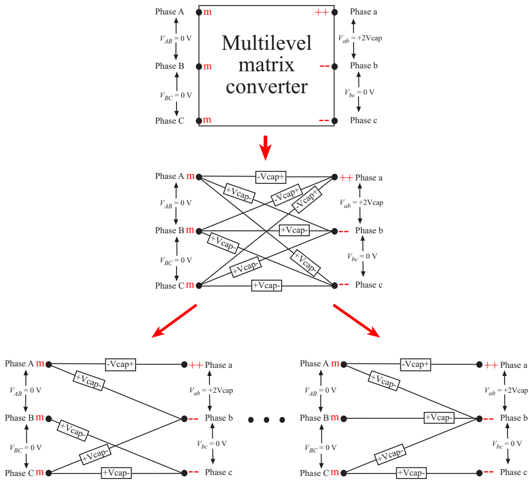
Figure 2.9: Generating valid switching combination: Case 3
