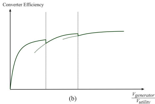
Figure 1.16: (a) Proposed capacitor voltage of the multilevel matrix converter in the wind turbine system, (b) prospective converter efficiency
