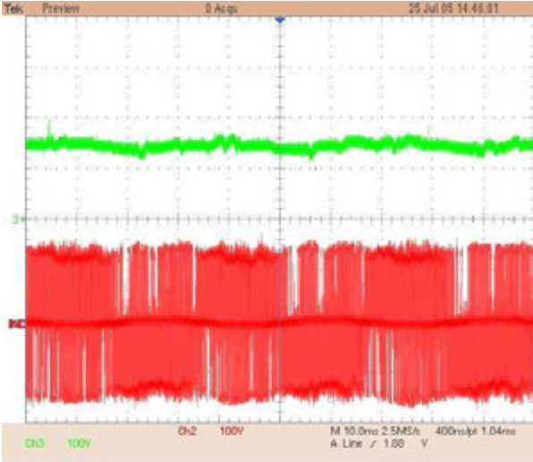
Figure 4.12: Waveforms of a capacitor voltage and an output PWM line-line voltage with capacitor voltage regulation
