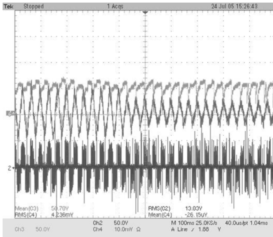
Figure 11.3: Experimental results of the matrix converter prototype when the output-line current changes from 1 A to 0.5 A amplitude: Top trace: capacitor voltage Middle trace: output current Bottom trace: output line-to-line voltage
