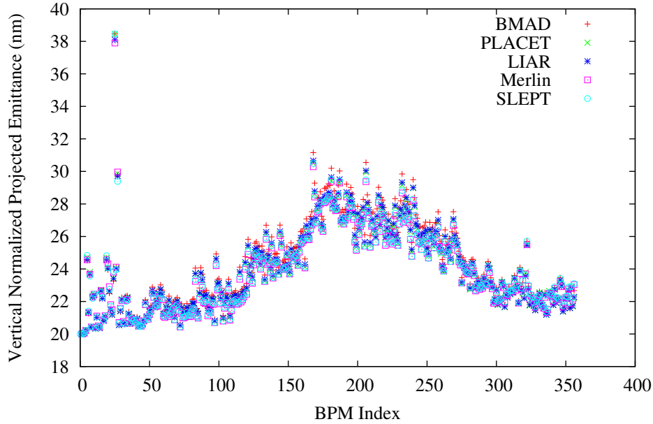
Figure 5: Emittance dilution after performing DFS in LIAR and reading misalignments and corrector settings into the other codes.
