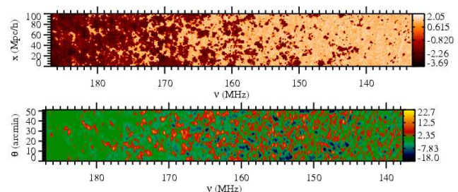
Fig. 1.— Large-scale geometry of reionization and the large local variations in reionization history as seen at redshifted 21-cm line: (top) \lg(\delta T_b) and (bottom) \delta T_b smoothed with 3' compensated Gaussian beam.
