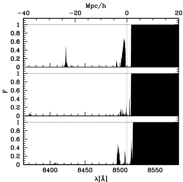
Fig. 4.— Ly- \alpha sources at redshift z = 6.0 : Transmission factor along sample lines-of-sight vs. \lambda/\text{comoving} distance from the most massive galaxy in the computational volume. There is significant transmission in the proximity zone and transmission gaps in the mean IGM away from the source. Gas infall results in some absorption red-ward of the line center.
