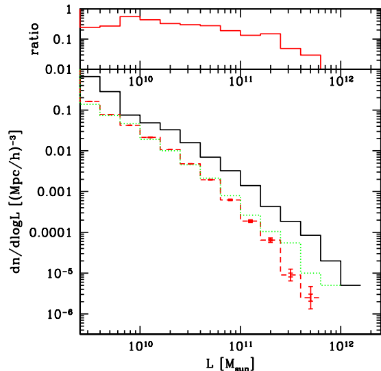
Fig. 5.— Ly- \alpha sources at redshift z = 6.0 : Luminosity function without (black) and with absorption included (red). For reference, the green, dotted line shows the result suppressing each source by 50%, which would be the case if e.g. all of the blue wing of the emission line, but none of the red wing is absorbed.
