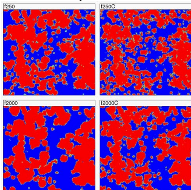
Fig. 1.— Large-scale geometry of reionization and the large local variations in reionization history as seen at redshifted 21-cm line: (top) \lg(\delta T_b) and (bottom) \delta T_b smoothed with 3' compensated Gaussian beam.
