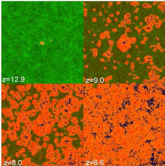
Fig. 3.— The reionization history of a high density peak. The images are centered on the most massive (at z = 6 ) halo in our computational volume and are of size 100 h^{-1}\text{Mpc} to the side. The snapshots are (left to right): z = 12.9 , z = 9.0 , z = 8.0 , and z = 6.6 . The underlying cosmological density field (dark, green) is superimposed with the ionized fraction (light, orange) and the ionizing sources (dark, blue dots).
