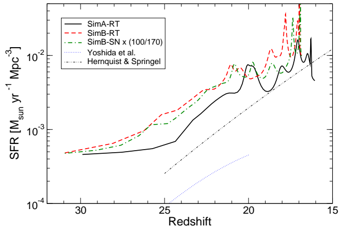
FIG. 2.— Comoving star formation rate in units of M_{\odot} \text{yr}^{-1} \text{Mpc}^{-3} . The lines representing the simulation data have the same meaning as in Figure 1. The crosses show at which redshifts stars form. The rates in SimB-SN are scaled for the same reason as in Figure 1. For comparison, we overplot the star formation rates from Hernquist & Springel (2003) in atomic hydrogen line cooling halos and Yoshida et al. (2003) for 100M_{\odot} Pop III stars.
