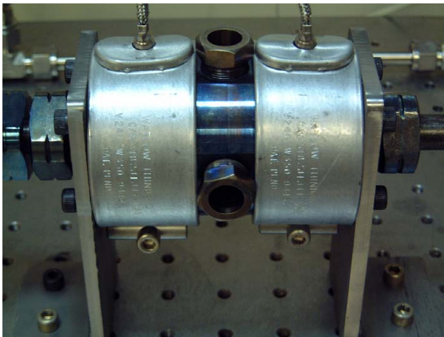
Figure 13. View cell.
