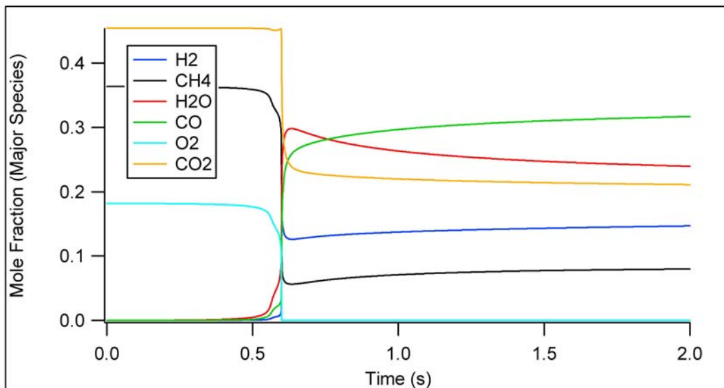
Figure 26. High pressure flame at 17 atm and \text{CH}_4:\text{O}_2 = 2 with \text{CO}_2 in the gas feed with no steam. Top) soot precursors, Bottom) syngas products.
