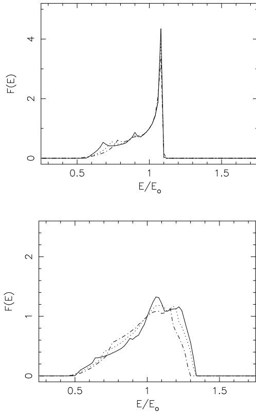
Fig. 8. Profiles of lines from accretion tori with aspect ratios corresponding to rotation velocity power-law indices n = 0.232 , 0.18 and 0.15 (represented by solid line, dotted line and dot-dashed line respectively). The spin parameter of the central black hole is a = 0.998 and the radius of Keplerian rotation is r_k = 8R_g . The tori have emissivity power-law index of -2 . The viewing inclination angles of the tori are 45^\circ (top panel) and 85^\circ (bottom panel). The normalisation is such that the flux F(E) = 1 at E/E_0 = 1 , where E_0 is the line centre energy in the rest-frame.
