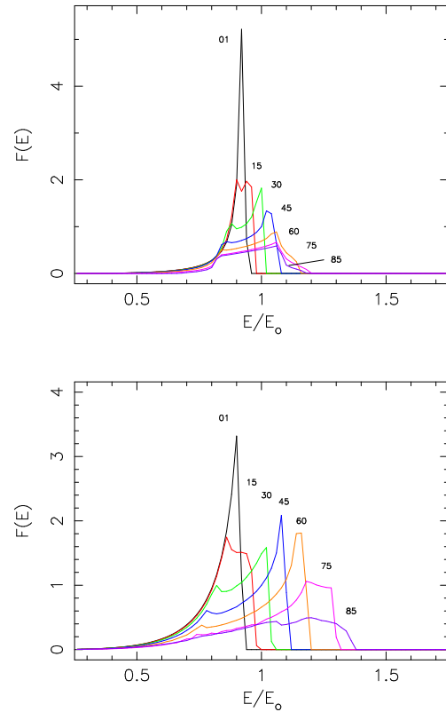
Fig. 16. Profiles of emission lines from accretion tori viewed at inclination angles i = 1^\circ, 15^\circ, 30^\circ, 45^\circ, 60^\circ, 75^\circ and 85^\circ . The radial emissivity power-law index is -2 . The radius of Keplerian rotation is r_k = 1.3R_g , and the spin parameter of the central black holes is a = 0.998 . The rotational velocity power law indices are n = 0.2 (top) and 0.01 (bottom). The normalisation is such that F(E) = 1 at E/E_0 = 1 for i = 45^\circ .
