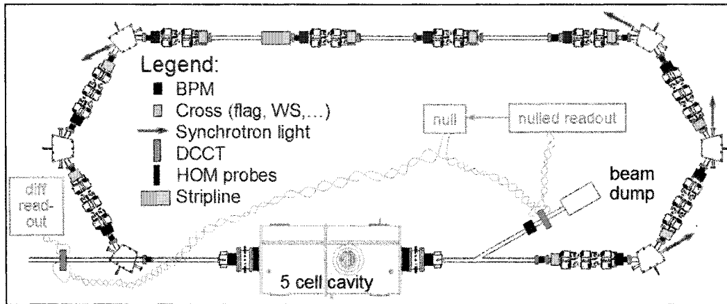
Figure 2: Layout of ERL Recirculation Loop diagnostics
