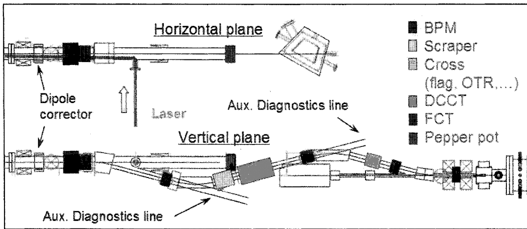
Figure 1: Layout of ERL Injector Diagnostics
