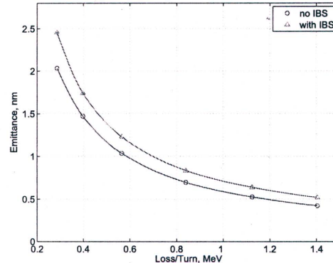
Figure 4: Emittance vs energy loss per turn
