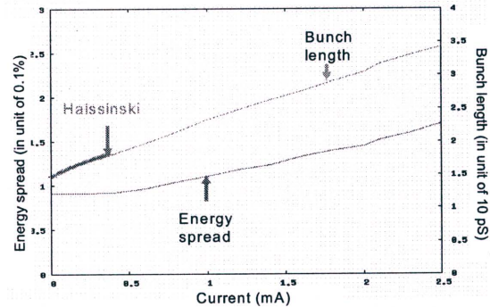
Figure 1: Bunch length and energy spread vs current
