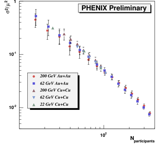
Figure 7: Multiplicity fluctuations for inclusive charged hadrons in the transverse momentum range 0.2 < p_T < 0.75 GeV/c in terms of \sigma^2/\mu^2 as a function of N_{\text{participants}} for 200 GeV Au+Au, 62 GeV Au+Au, 200 GeV Cu+Cu, 62 GeV, and 22 GeV Cu+Cu collisions. The data have been scaled by factors of 1.0, 0.73, 1.43, 0.73, and 1.0, respectively, in order to emphasize the universal scaling of all species. The dashed curve is a power law fit as described in the text.
