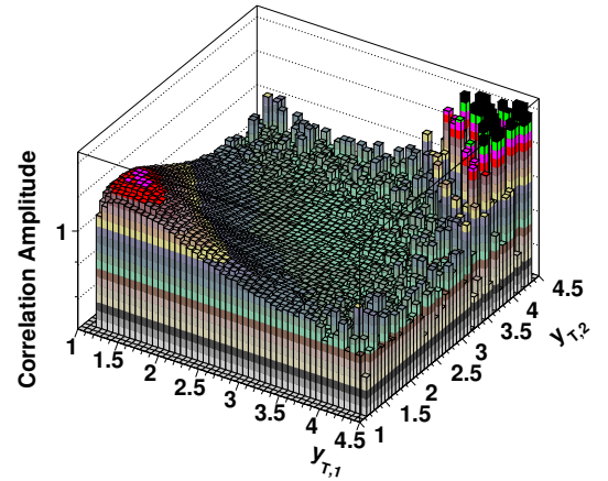
PHENIX Preliminary: 200 GeV Au+Au, 0-5% Centrality, Like-Sign, Near-Side
