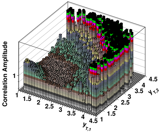
PHENIX Preliminary: 200 GeV d+Au, Min. Bias, Like-Sign, Near-Side
